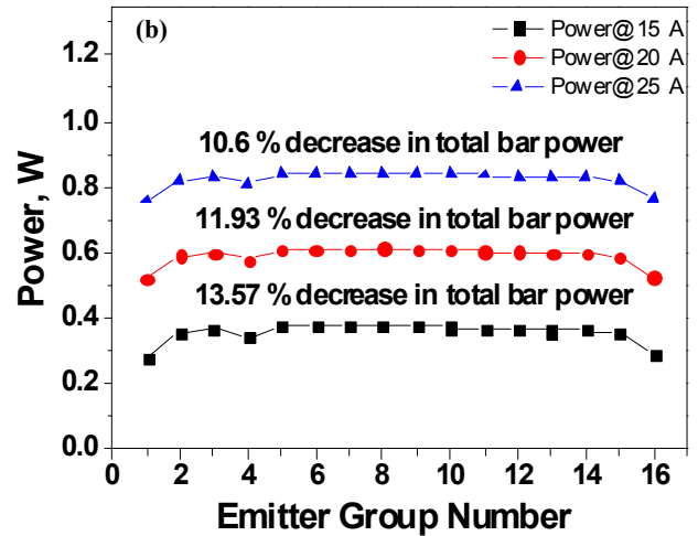
Figure 8. Comparison of power distribution profiles of bar 16022: (a) experimental output power; (b) emulated output power.
