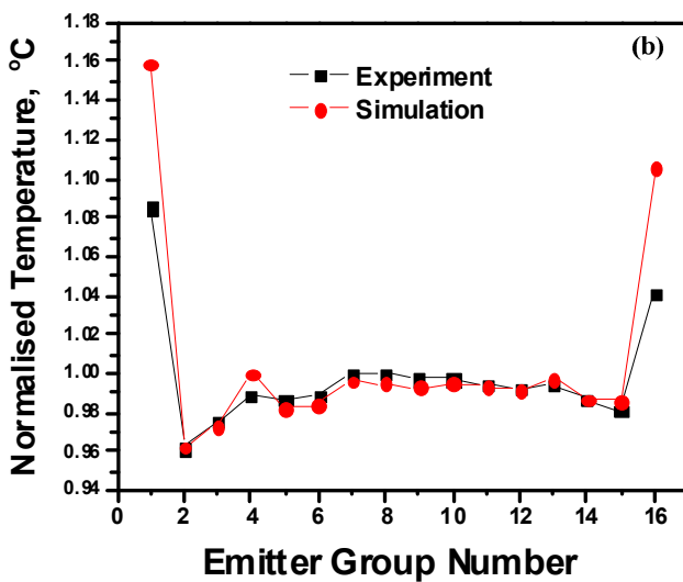
Figure 7. Simulated output power and temperature profiles of Bar 16022; (a) modified defect levels at edge emitters by a factor of 3, (b) normalised temperature without edge emitters.
