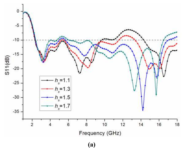
Figure 2. Simulated S_{11} with (a) one slot, and (b) two slots with l_1 = 6 mm
